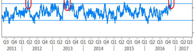
Relative Strength Index (measures momentum)
